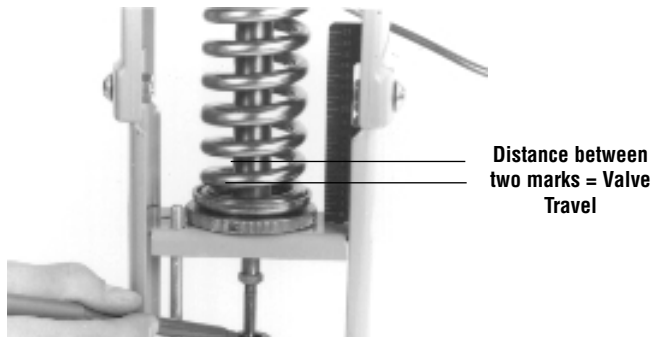
14. VALVE TRAVEL MEASUREMENT
