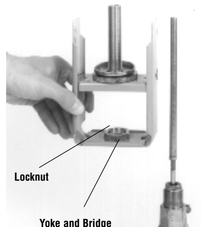
9. LIFT OFF YOKE AND BRIDGE
