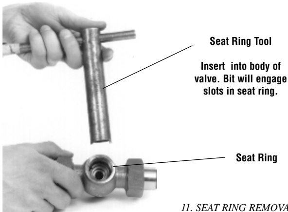
11. SEAT RING REMOVAL
