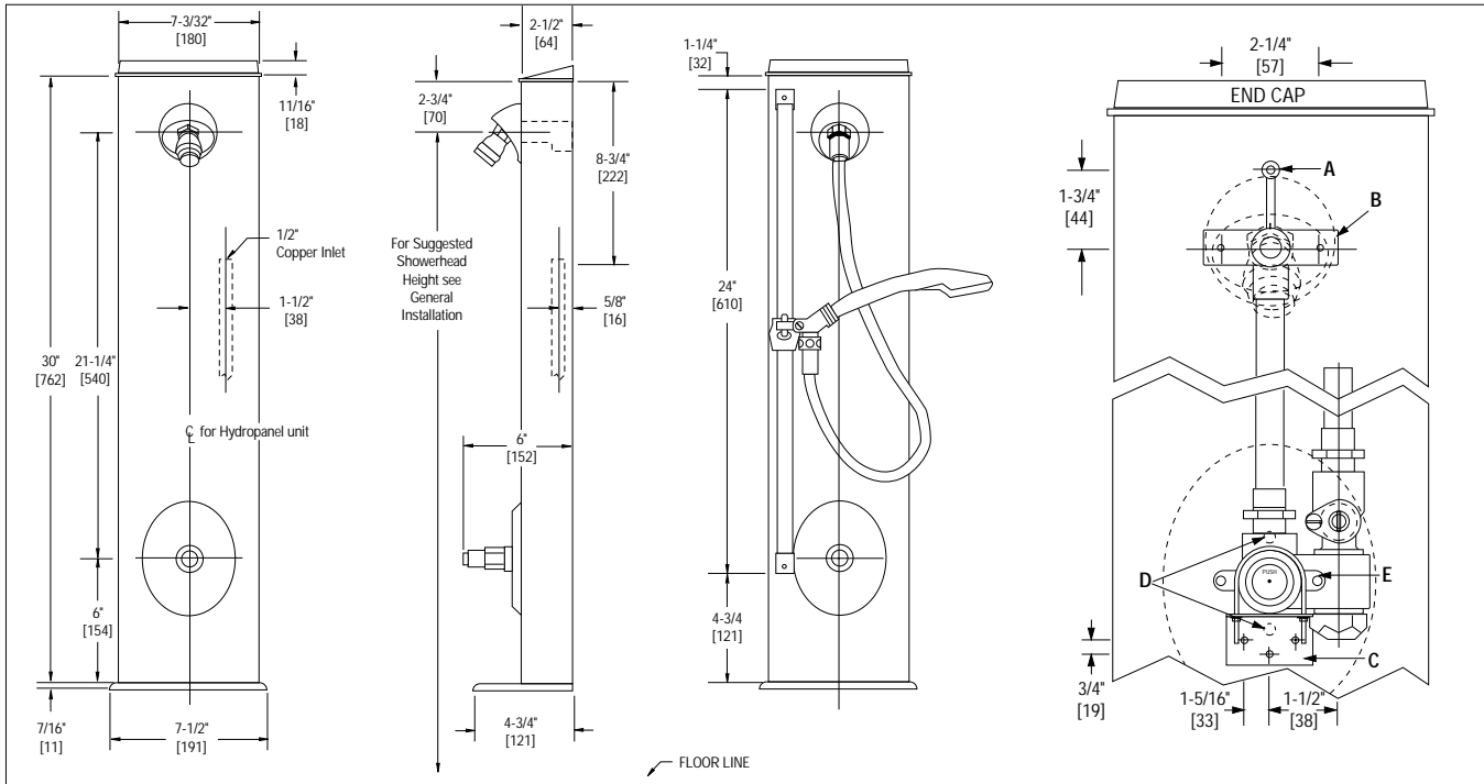
Figure 4: Piping Assembly, Hydropanel II Series 450-4002M.
